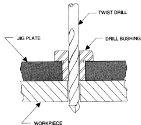
Fig-1: jig guides the tool, with a bushing.
