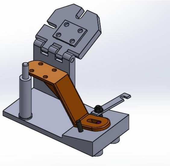
Fig-12: jig after workpiece placed
