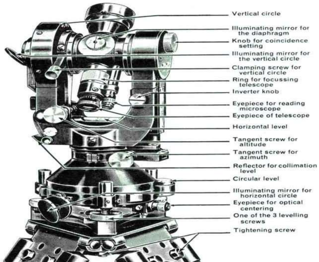
TRANSIT THEODOLITE
