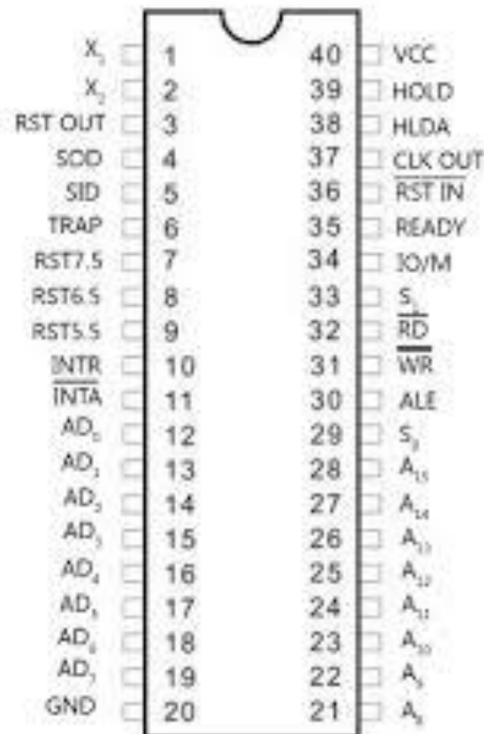
Fig. No. 2:- Pin Diagram of 8085
